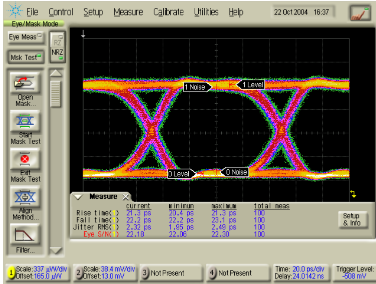
Typical 10Gbps unfiltered eye diagram of D-150 (20ps/div)
