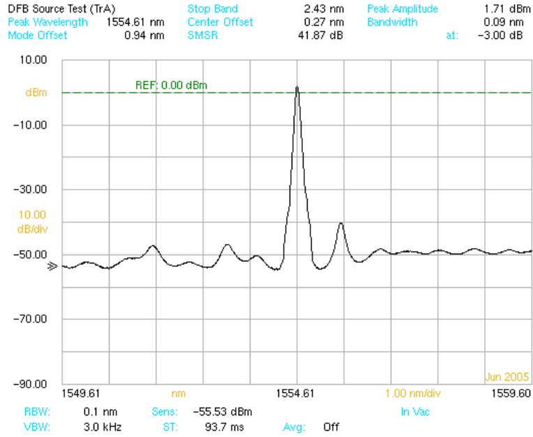
Typical D-150 Output Spectrum.
