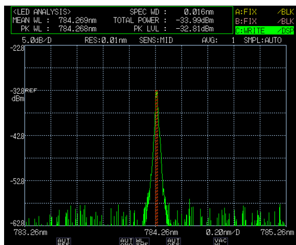
785 nm SS Laser Spectrum @ 25 deg C
