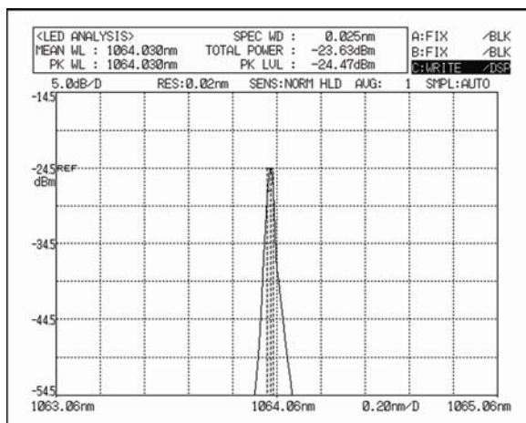
1064 nm SS Laser Spectrum @ 25 deg C
