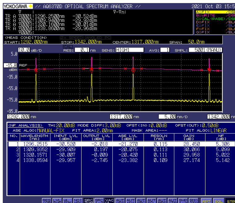
Optical gain and NF for 4 wavelengths input
